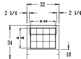
SW32-12M TOP VIEW
