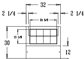
SW32-8 TOP VIEW
