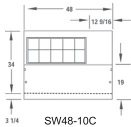
SW48-10C
